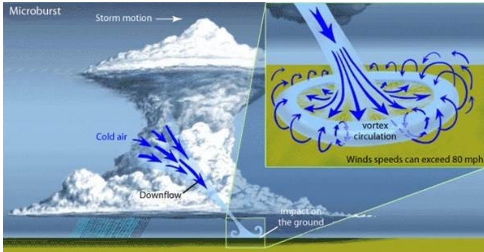
Figure 2C.2.7: Microburst
